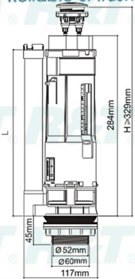
A2412 Dual Flush Valve
